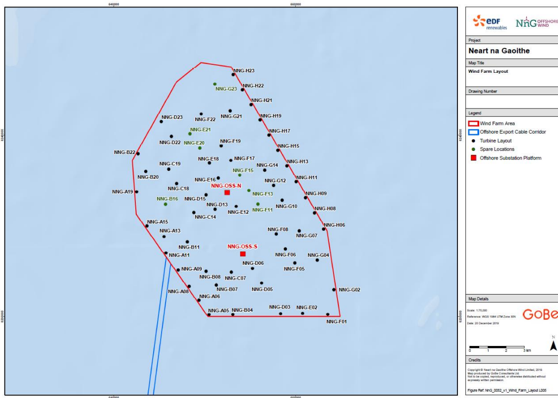
Figure 1 – NnG Offshore Wind Farm Turbine Locations
