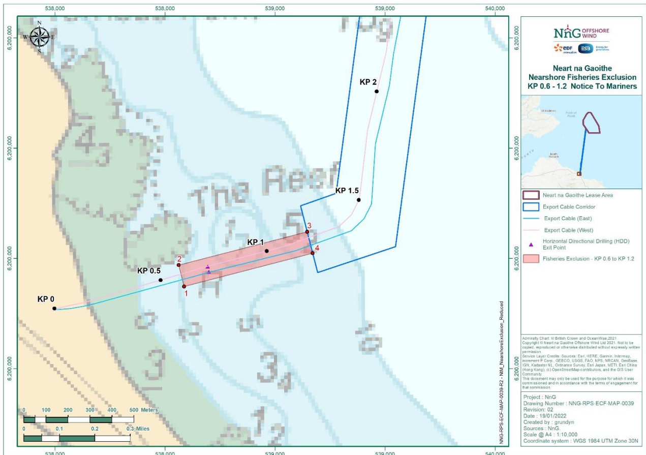
Figure 1 - Nearshore export cable safe advisory avoidance area
