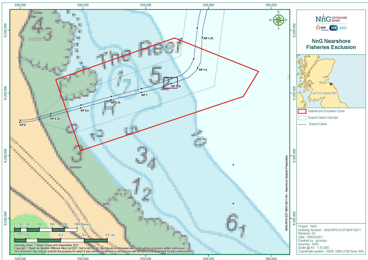
Figure 1 - Nearshore export cable exclusion areas
