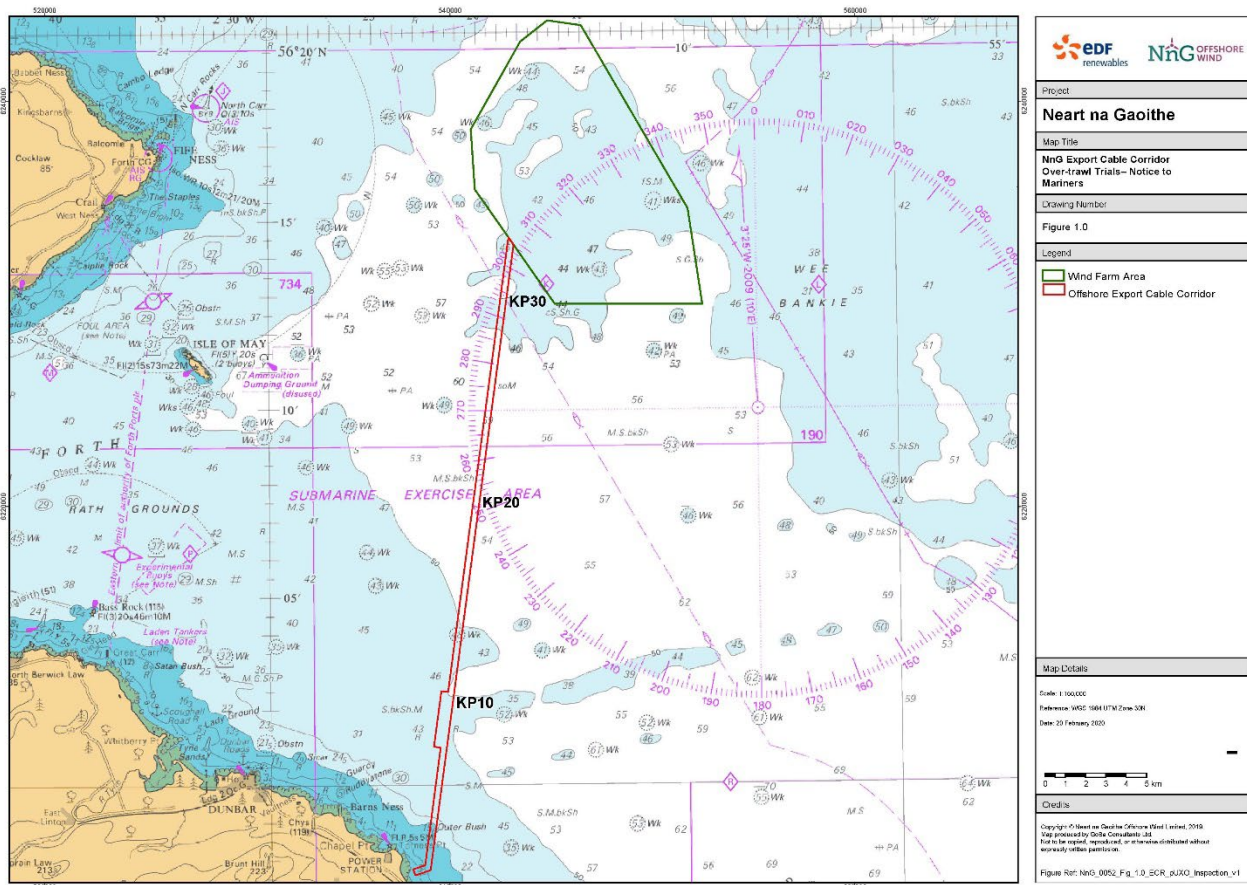
Figure 1 - Location of Export Cable Over-trawl trials
