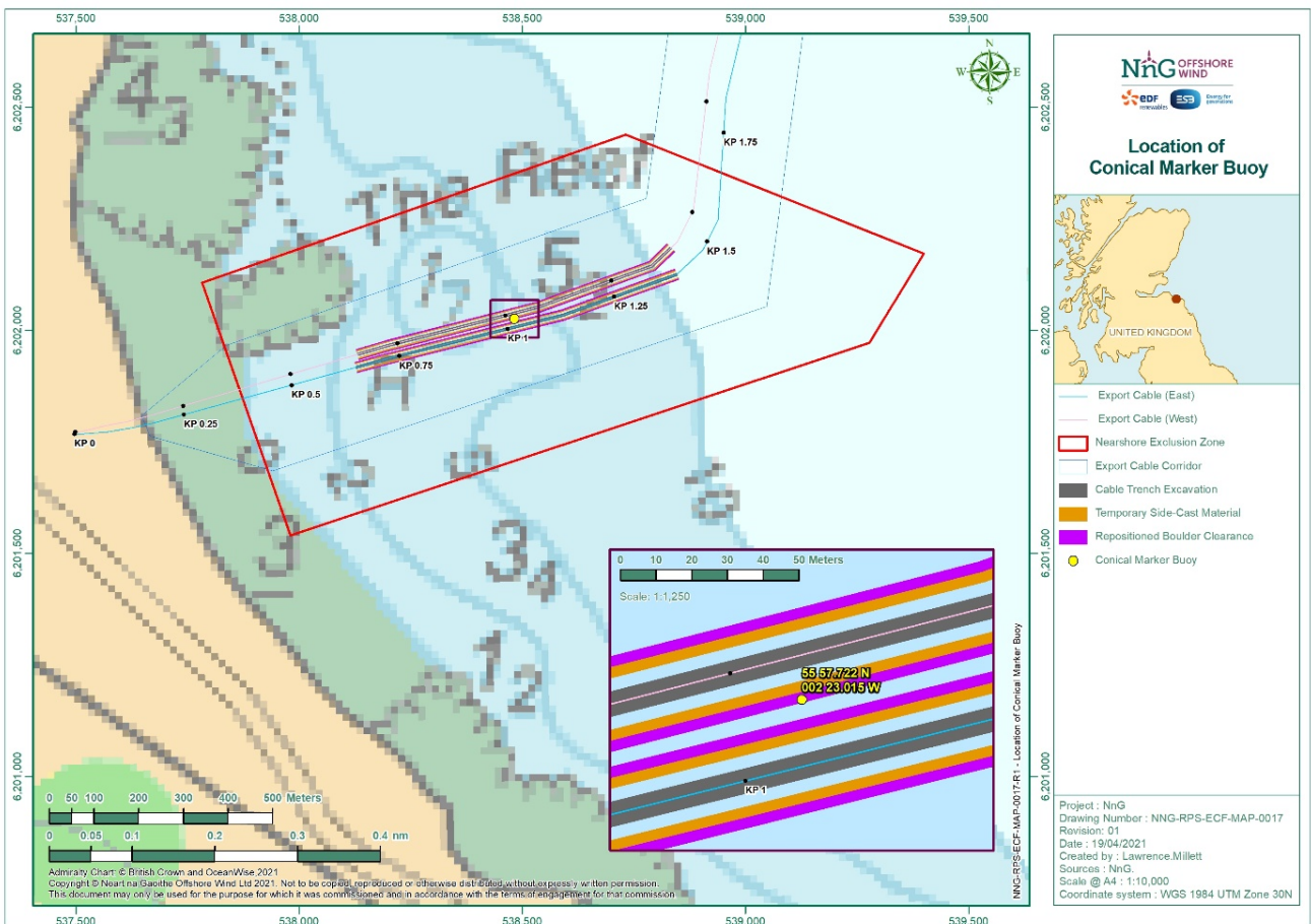
Figure 1 – Location of conical marker buoy
