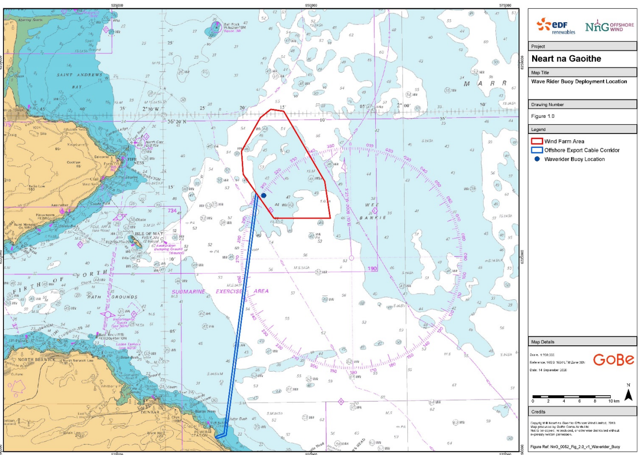
Figure 1 Wave Rider Buoy Location
