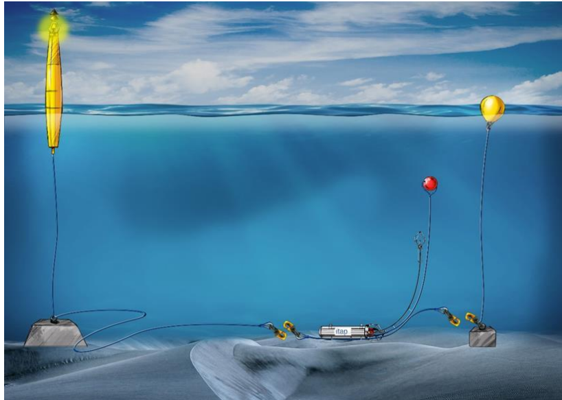
Figure 2 Schematic of mooring
