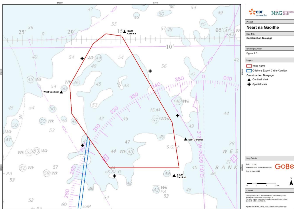
Figure 1 Location of Construction Navigation Buoys
