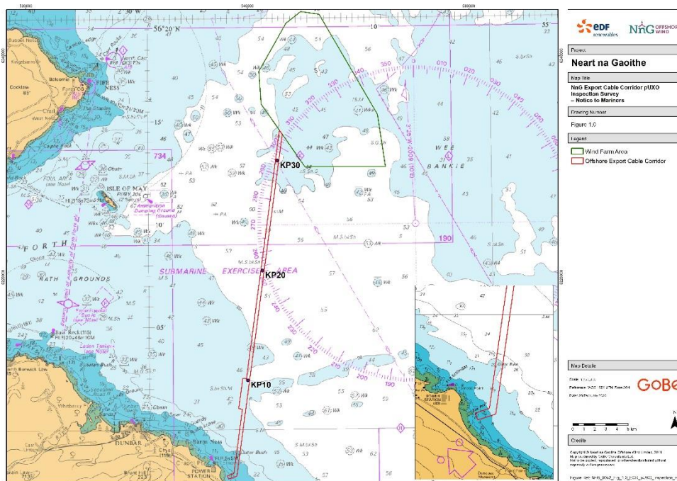
Figure 1 pUXO Inspection Survey Area – Export Cable Corridor
