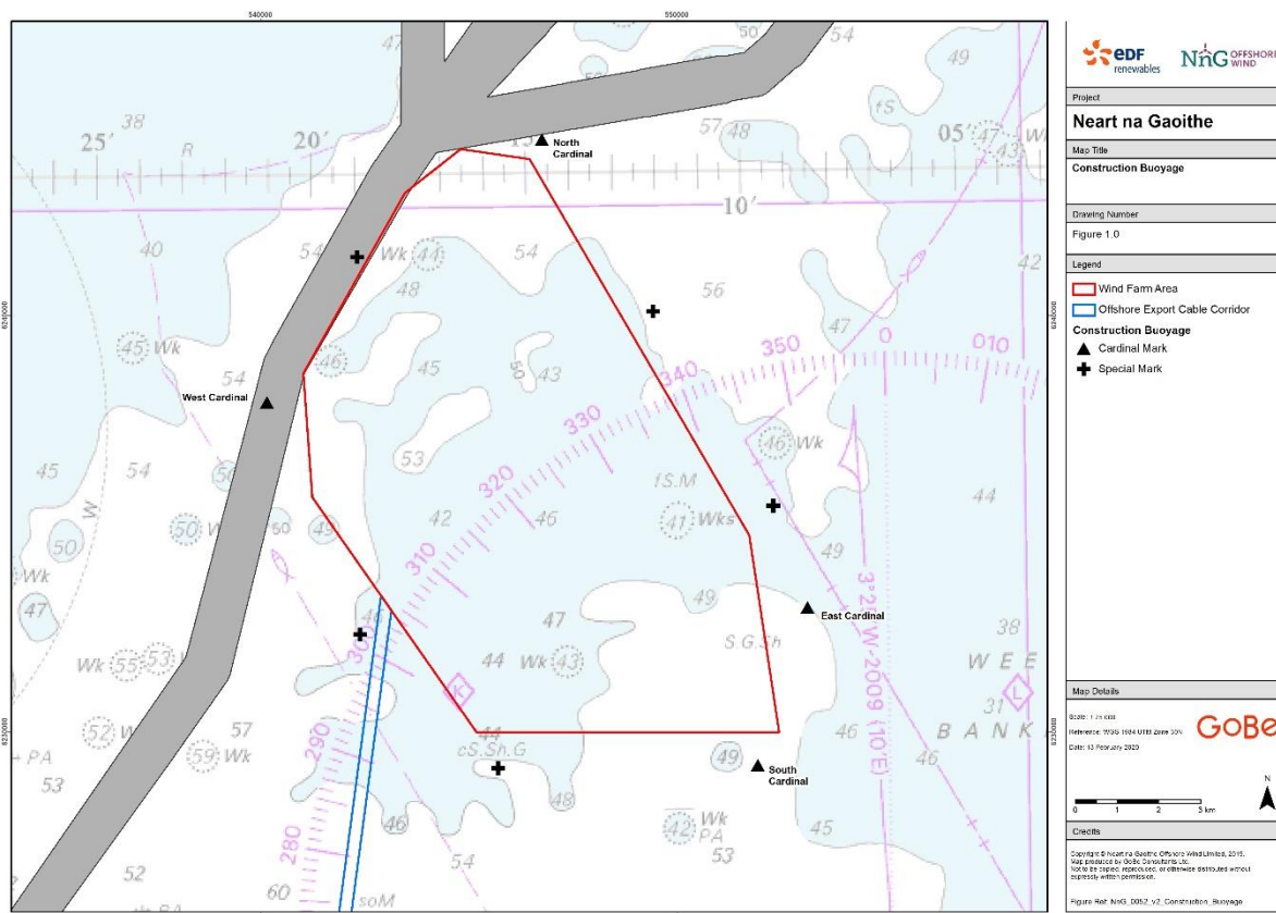
Figure 1 Location of Construction Navigation Buoys
