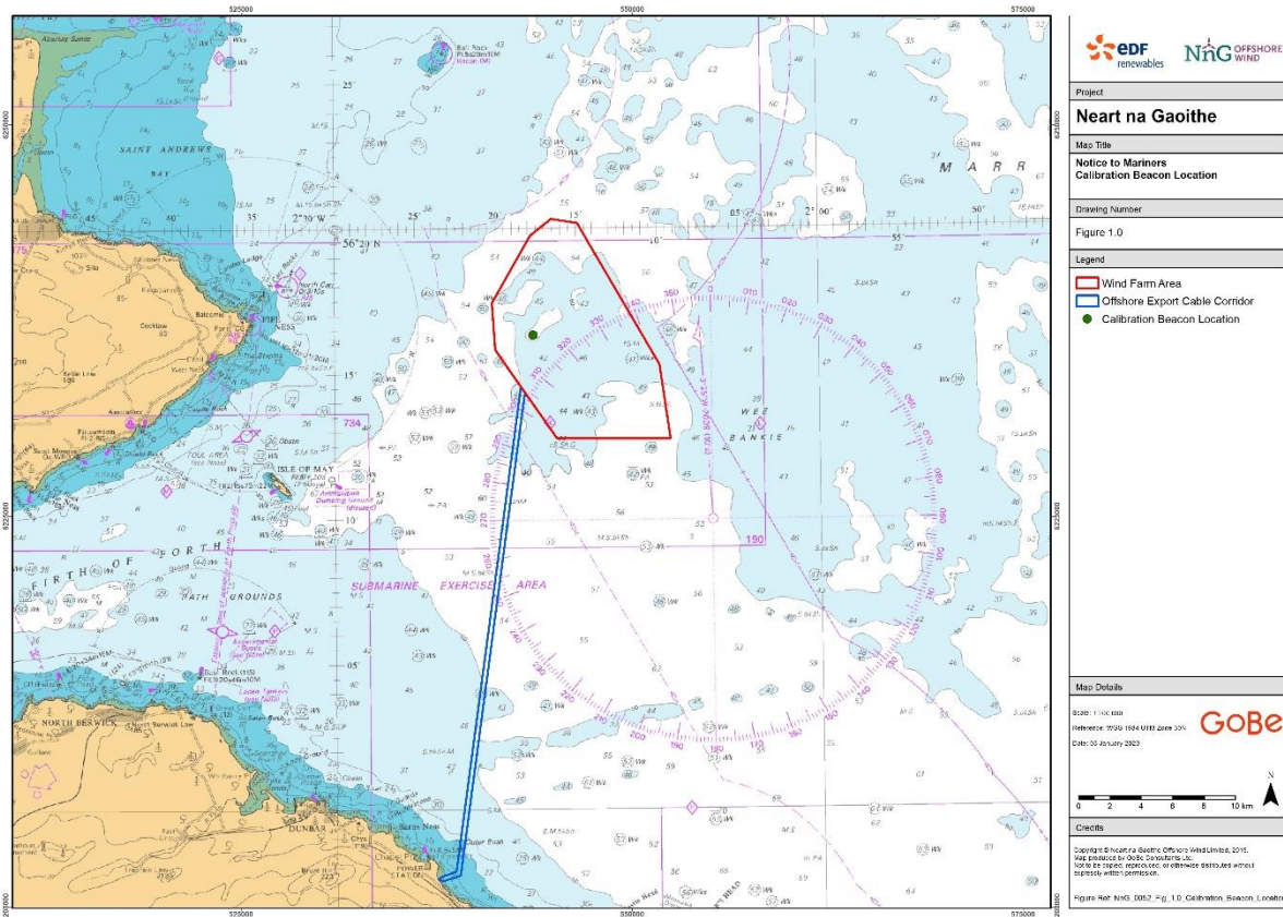
Figure 1 Location of calibration beacon (USBL Transponder 2310) within the Neart na Gaoithe wind farm boundary
